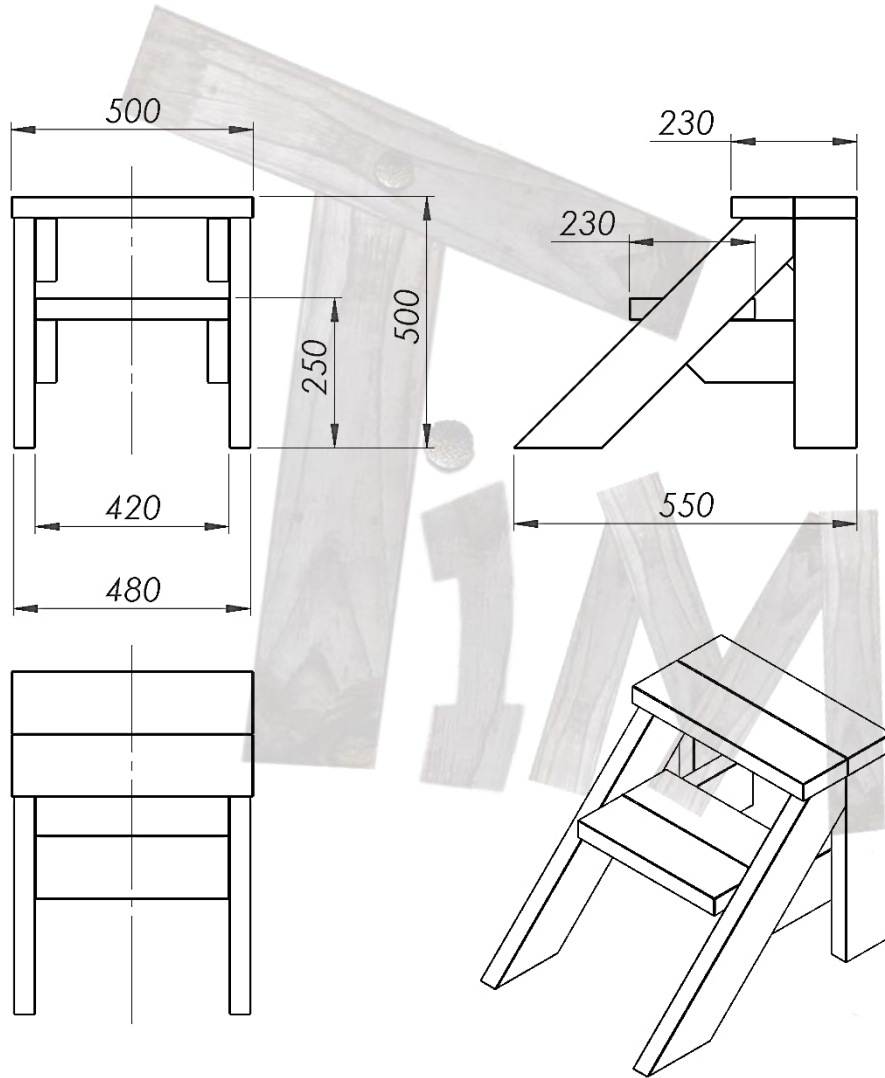
"B" type stairs
