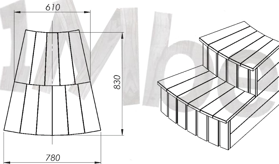
"A" type stairs
