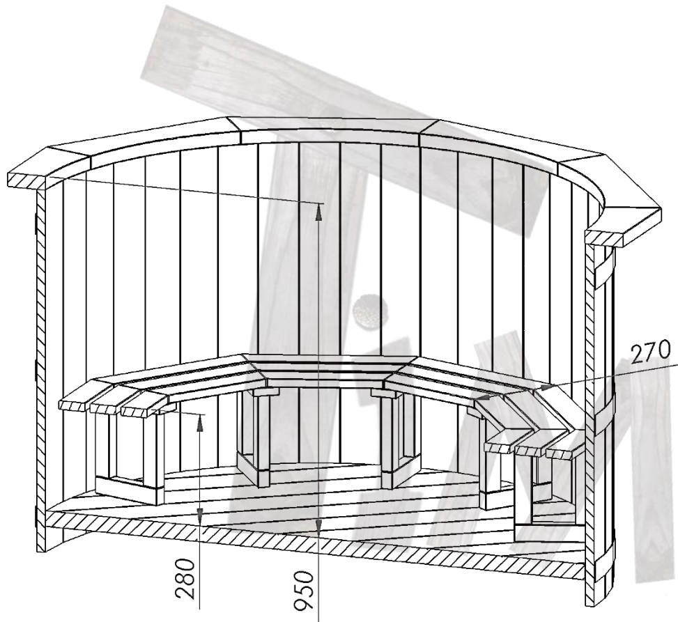
Wooden benches in 360 degrees (for electric and external heaters)
