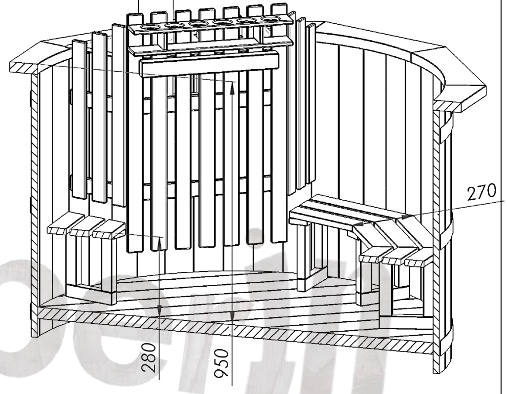
Wooden benches in 270 degrees (for internal heater)
