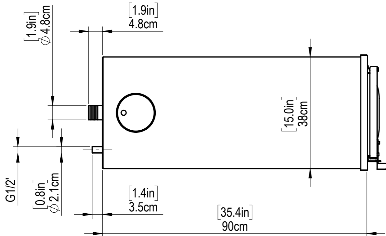
Combustion chamber cross-section dimensions
