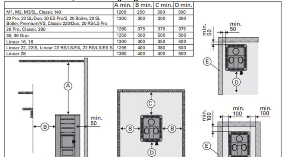
Figure 1 Safety distances (all dimensions in millimeters)
