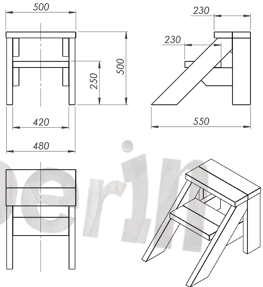
"B" type stairs
